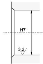
相配座孔 Mating Housing
